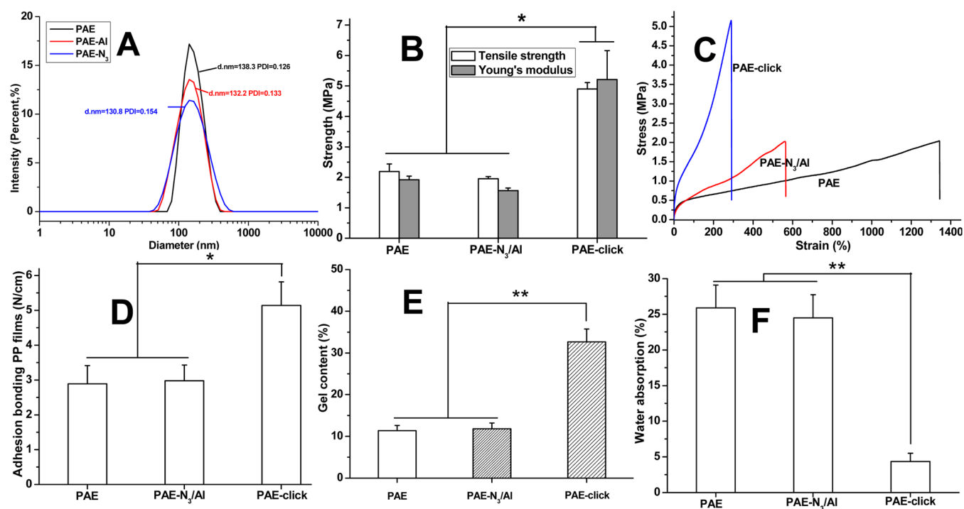
Figure 7. (A) Particle sizes and particle size distributions (PDI) of PAE, PAE-Al, and PAE-N 3 emulsions. (B) Tensile strengths, Young's moduli, (C) stress-strain curves, (D) adhesion properties, (E) gel contents, and (F) water-resistance properties of PAE, Physically mixed click-suitable PAE (PAE-N 3 /Al), and click cross-linked PAE (PAE-click). * p < 0.05, ** p < 0.01.
