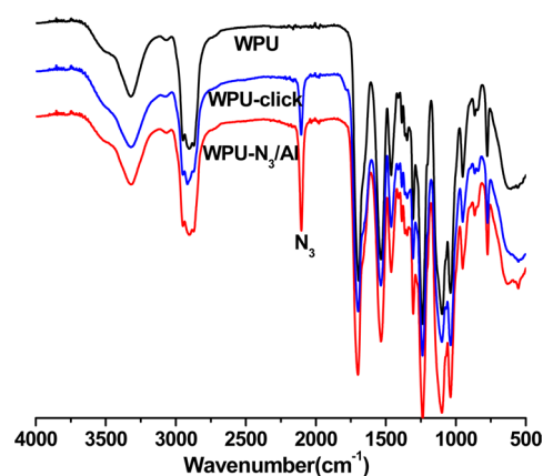
Figure 3. FTIR spectra of WPU, physically mixed click-suitable WPU (WPU-N 3 /Al), and click cross-linked WPU (WPU-click).
