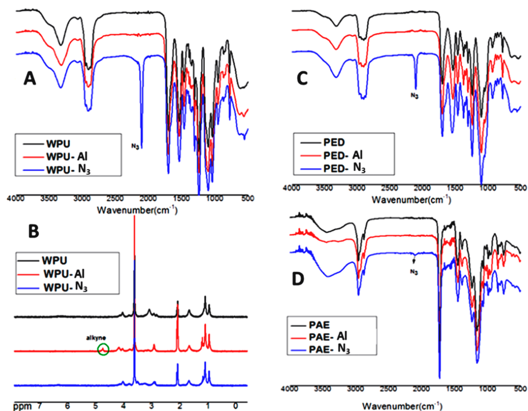
Figure 2. FTIR spectra (A) and 1 H NMR spectra (B) of nonclick waterborne polyurethane (WPU), waterborne polyurethane with side alkyne groups (WPU-Al), and waterborne polyurethane with side azide groups (WPU-N 3 ). FT-IR spectra of (C) PED, PED-Al, and PED-N 3 and (D) PAE, PAE-Al, and PAE-N 3 .
