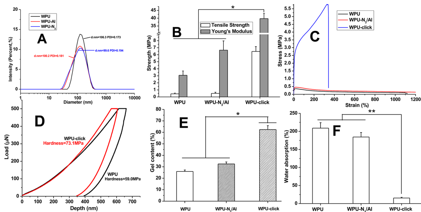
Figure 4. (A) Particle sizes and particle size distributions (PDI) of WPU, WPU-Al, and WPU-N 3 suspensions. (B) Tensile strength, Young's moduli, (C) stress-strain curves, (D) hardness (determined by nanoindentation test), (E) gel contents, and (F) water-resistance properties of WPU, physically mixed click-suitable WPU (WPU-N 3 /Al), and click cross-linked WPU (WPU-click). * p < 0.05, ** p < 0.01.
