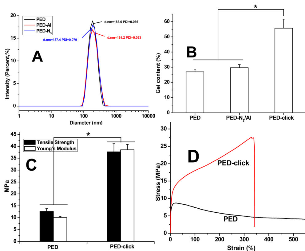
Figure 6. (A) Particle sizes and particle size distributions (PDI) of PED, PED-Al, and PED-N 3 suspensions. (B) Gel contents of PED, physically mixed click-suitable PED (PED-N 3 /Al), and click cross-linked PED (PED-click). (C) Tensile strengths, Young's moduli, and (D) stress-strain curves of PED and click cross-linked click-suitable PED (PED-click). * p < 0.05.
