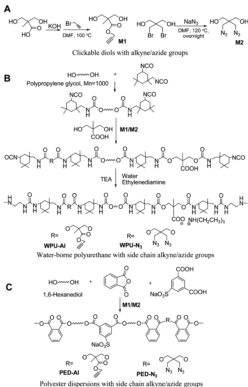
Scheme 1. Schematic Representation of Click Monomers and WPU and PED Click Cross-Linking. (A) Synthesis of Click-Suitable Diol Monomers (M1, M2); (B) Polymerization of WPU-N 3 or WPU-Al, (C) PED-N 3 or PED-Al
